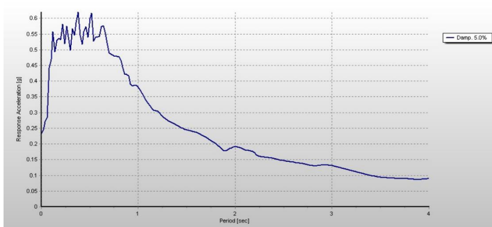
Figure 7 Spectrum Response Image Output from Seismosignal Software
