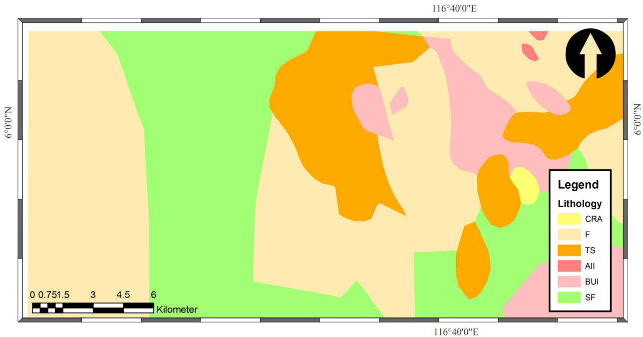
Figure 2. The lithological units distribution in the study area.
