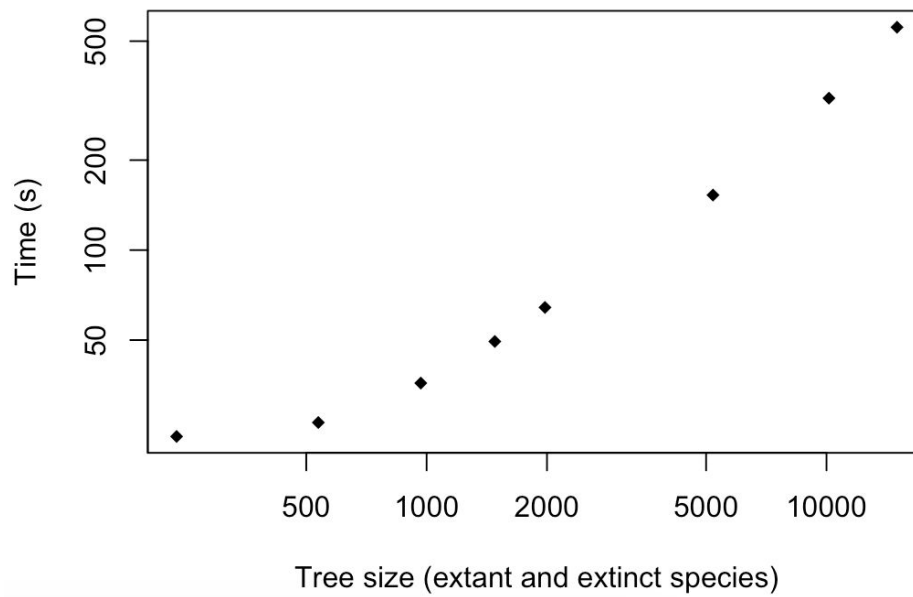
Figure S2. Computing time for different simulation in a computer with a 3,4 GHz Intel Core i5 processor. The rates used were Duplication rate: 0.2, Transfer rate: 0.2, Loss rate: 0.6, Origination rate:0.05, Inversion rate: 0.2, Translocation rate: 0.2. The initial genome was composed of 500 genes. All extension rates were set to 1. Species trees were obtained using by setting Speciation rate: 1 and Extinction rate: 0.5.
