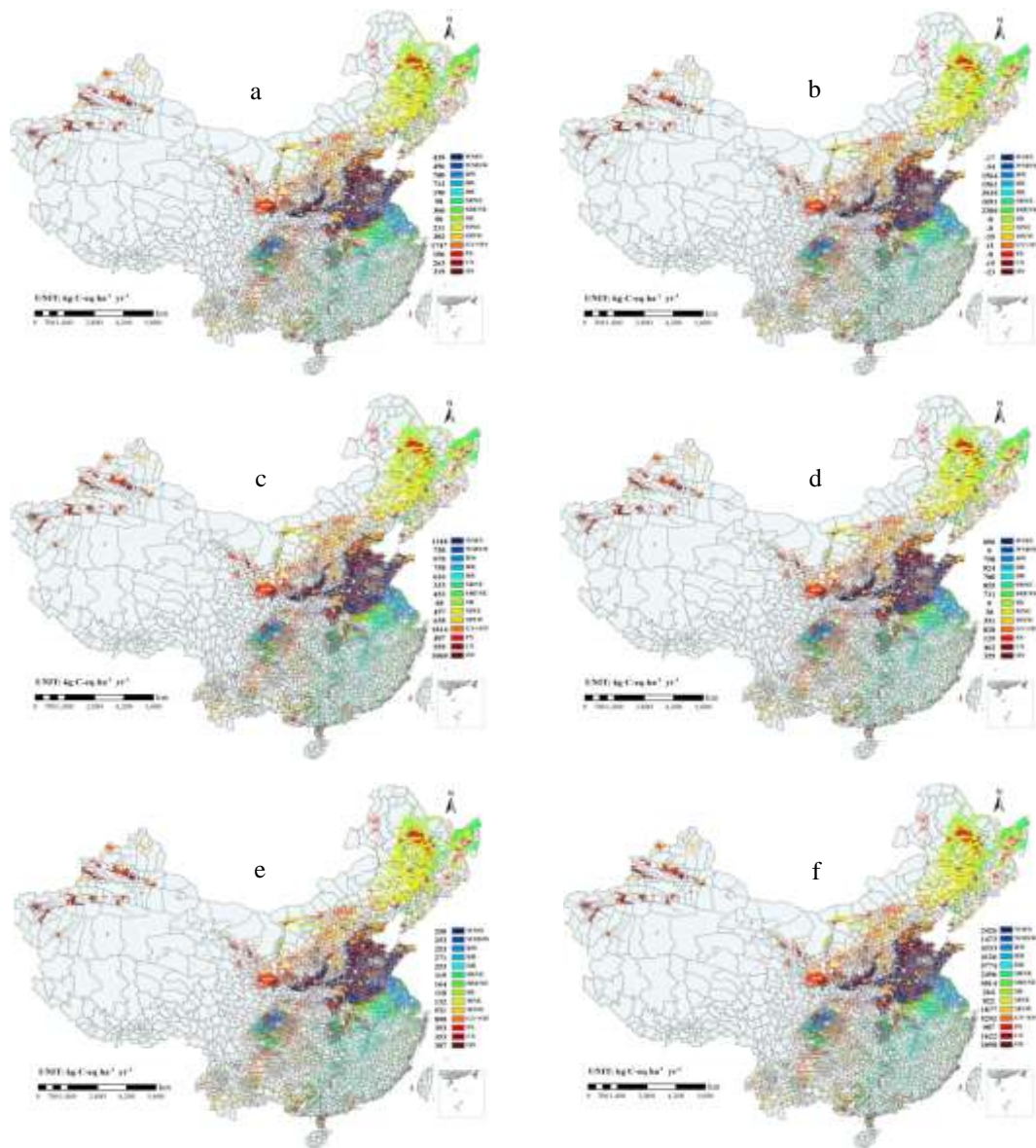
Fig. S1. Spatial pattern of GHG emissions ( \text{kg C-eq ha}^{-1} ) from \text{N}_2\text{O} emission (a), \text{CH}_4 emission (b), application of N fertilizer (c), power use for irrigation (d), other sources include \text{P}_2\text{O}_5 and \text{K}_2\text{O} fertilizer application, fuel in farm operation, pesticide and film mulch (e) and total GHG emissions from above sources (f) in Chinese cropping systems. WMN, WMSW, RW, RR, DR, SRNE, SRENE, SB, MNE, MNW, GV+OV, PS, CS, and OS represent winter wheat – summer maize double cropping system in Northern China, winter wheat – summer maize double cropping system in Southwestern China, rice – winter wheat double cropping system, rice – rapeseed double cropping system, double rice system, single rice system in Northeastern China, single rice system except for Northeastern China, soybean in Northeastern China, spring maize in Northeastern China, spring maize in Northern and Northwestern China, vegetable system, potato system, cotton system, and orchard system, respectively.
