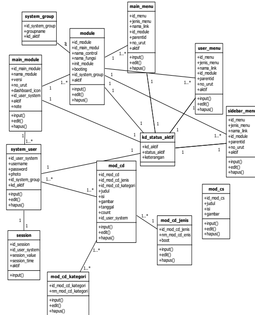
Gambar. 2 Class Diagram
