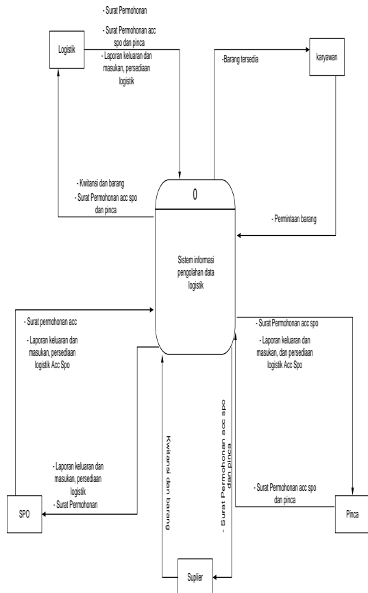
Gambar. 4 Context Diagram Sistem Pengolahan Data Logistik
