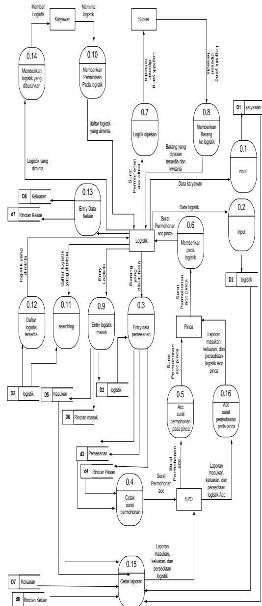
Gambar. 5 Data Flow Diagram Level 0
