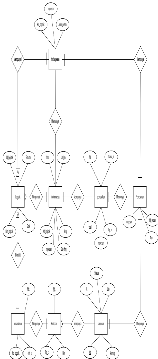
Gambar 6. Entity Relationship Diagram
