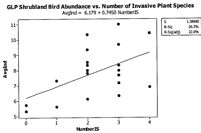
Figure 5. Regression of average individual shrubland birds on number of invasive shrub species. GLP 2006-2007 ( p = 0.015 ).
