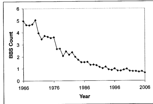
Figure 2. Abundance trends for Brown Thrasher ( Toxostoma rufum ) in New York State (BBS 2006)
