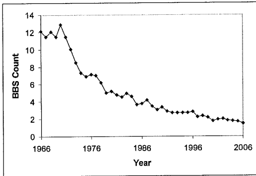
Figure 1. Abundance trends for Eastern Towhee ( Pipilo erythrophthalmus ) in New York State (BBS 2006)
