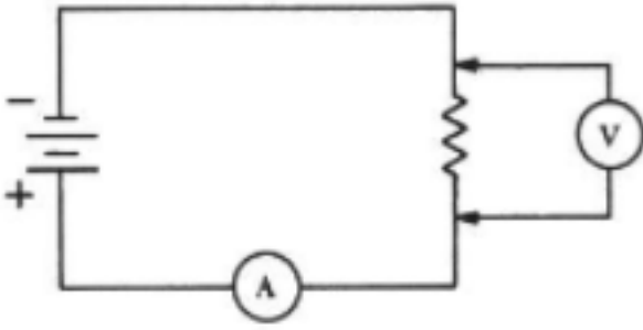
Figure 7. Simple circuit with one resistor, a voltmeter, and an ammeter.
