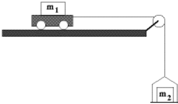
Figure 5. Modified Atwood's machine with a system consisting of a cart and a hanger with slotted masses.
