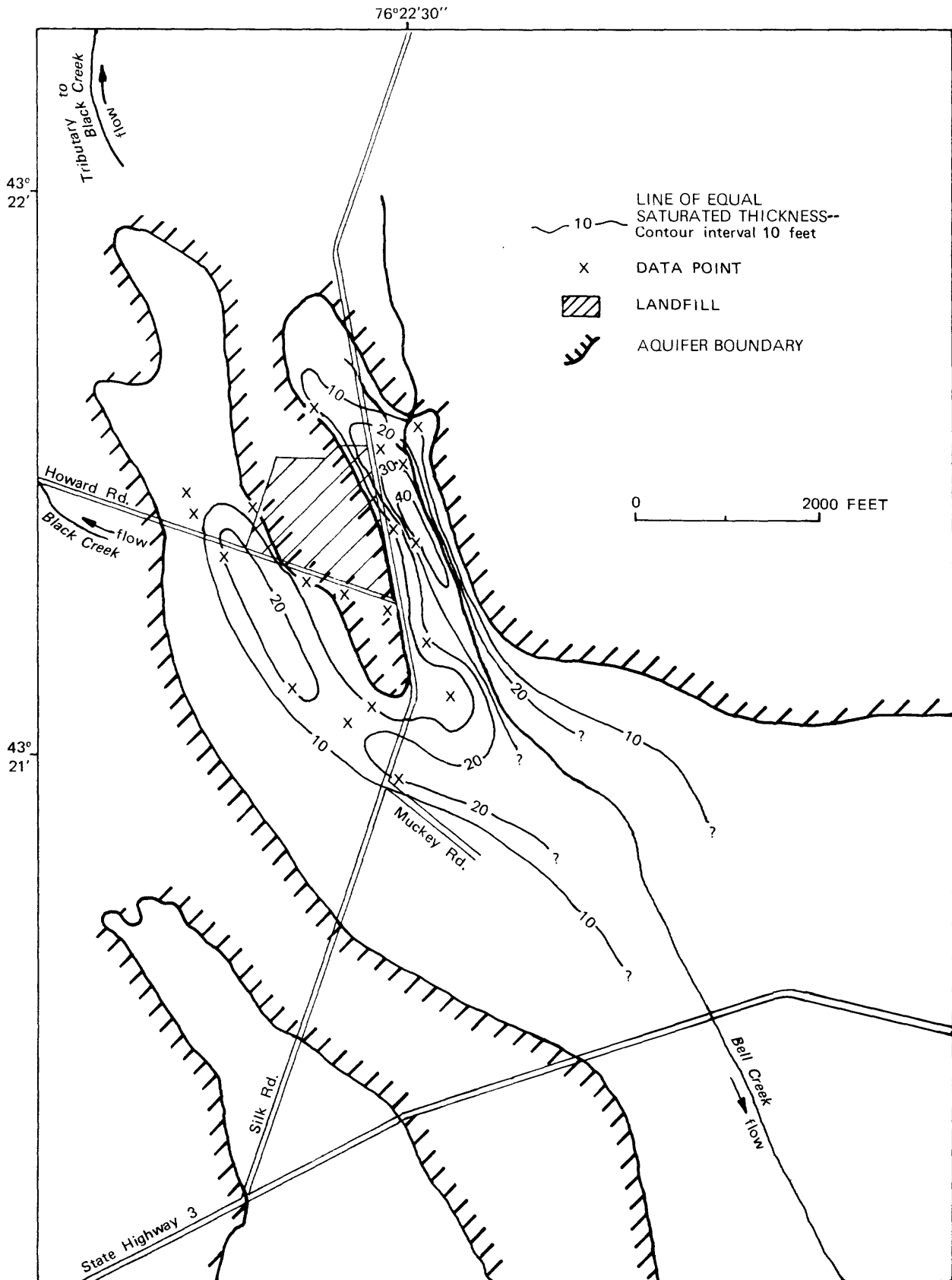
Figure 10.--Saturated thickness of sand and of sand and gravel aquifer in vicinity of landfill near Fulton. (Location is shown in fig. 2.)
