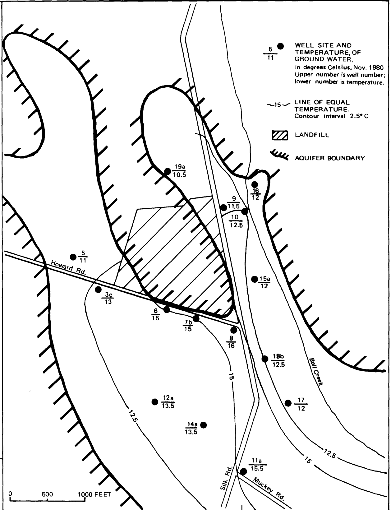
Figure 13B.--Temperature of ground water in vicinity of landfill near Fulton, November 1980. (Location is shown in fig. 9.)
