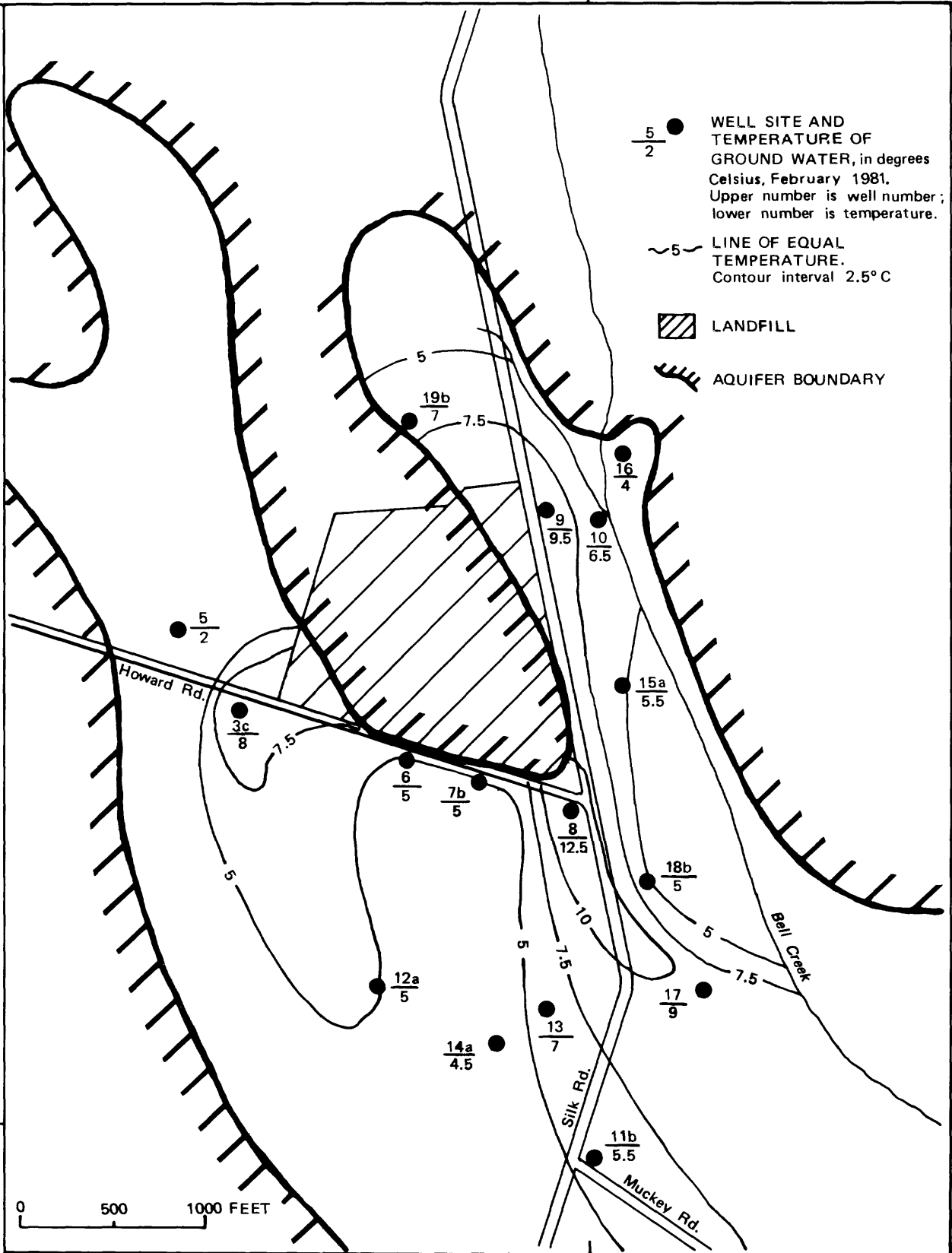
Figure 13C.--Temperature of ground water in vicinity of landfill near Fulton, February 1981. (Location is shown in fig. 9.)
