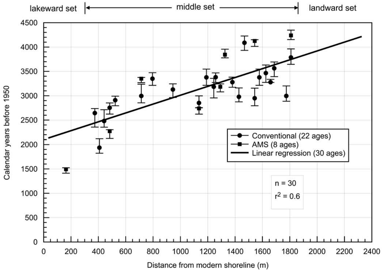
FIG. 5. Graph of calibrated ages versus distance from the modern shoreline. The regression line was used to calculate approximate ages for each beach ridge in the Tahquamenon Bay embayment.
