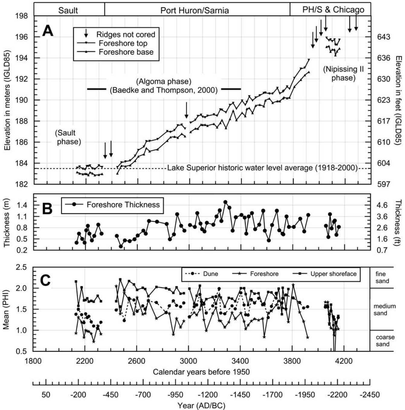
FIG. 6. Graph of (A) foreshore (top and base) elevation trends, (B) foreshore thickness, and (C) mean grain size of nearshore (foreshore and upper shoreface) and onshore (dune) facies per core versus calendar years before 1950 across the entire Tahquamenon Bay strandplain. Basal foreshore elevations in (A) indicate the relative elevation of the lake through time. (Note: Basal foreshore elevations in (A) are relative lake-level elevations only with respect to Tahquamenon Bay because vertical ground movement is not removed.)
