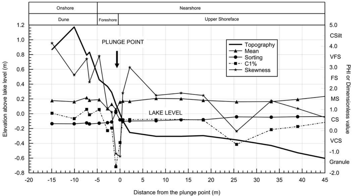
FIG. 2. Graph of onshore/nearshore topography and grain-size trends perpendicular to the modern shoreline at Tahquamenon Bay, Michigan. The profile extends across the modern beach and plunge point (land/water interface) and into the nearshore. The modern shoreline is eroding, producing a steep topographic profile on the landward part of the profile. Abbreviations along the second y-axis describe the grade of sediment (granular gravel to very coarse, coarse-, medium-, fine-, and very fine grained sands to coarse-grained silt).
