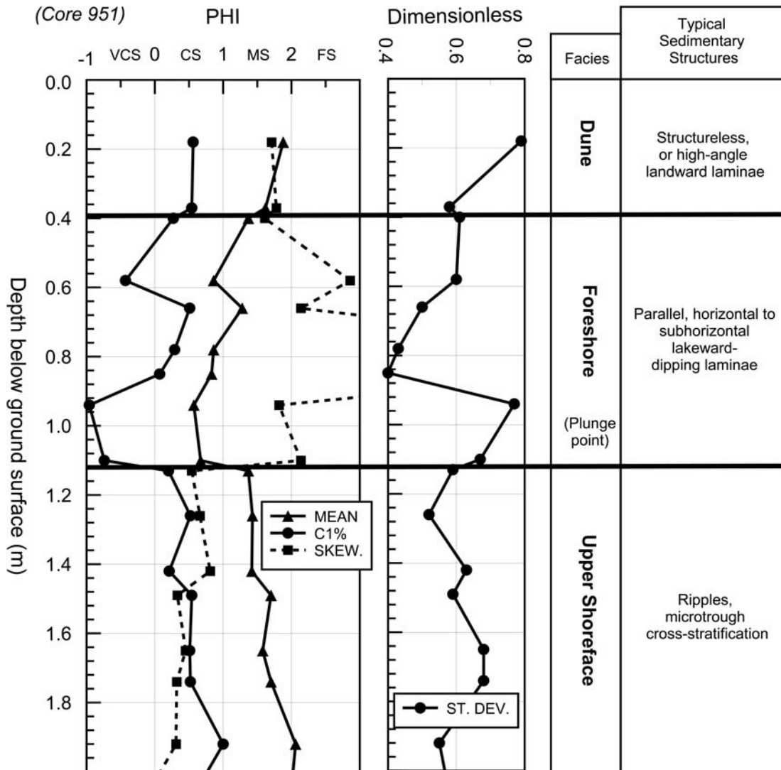
FIG. 3. Schematic diagram illustrating facies grain-size characteristics in core 951 with respect to depth and typical sedimentary structures in all cores. See Figure 2 for grain-size abbreviations.
