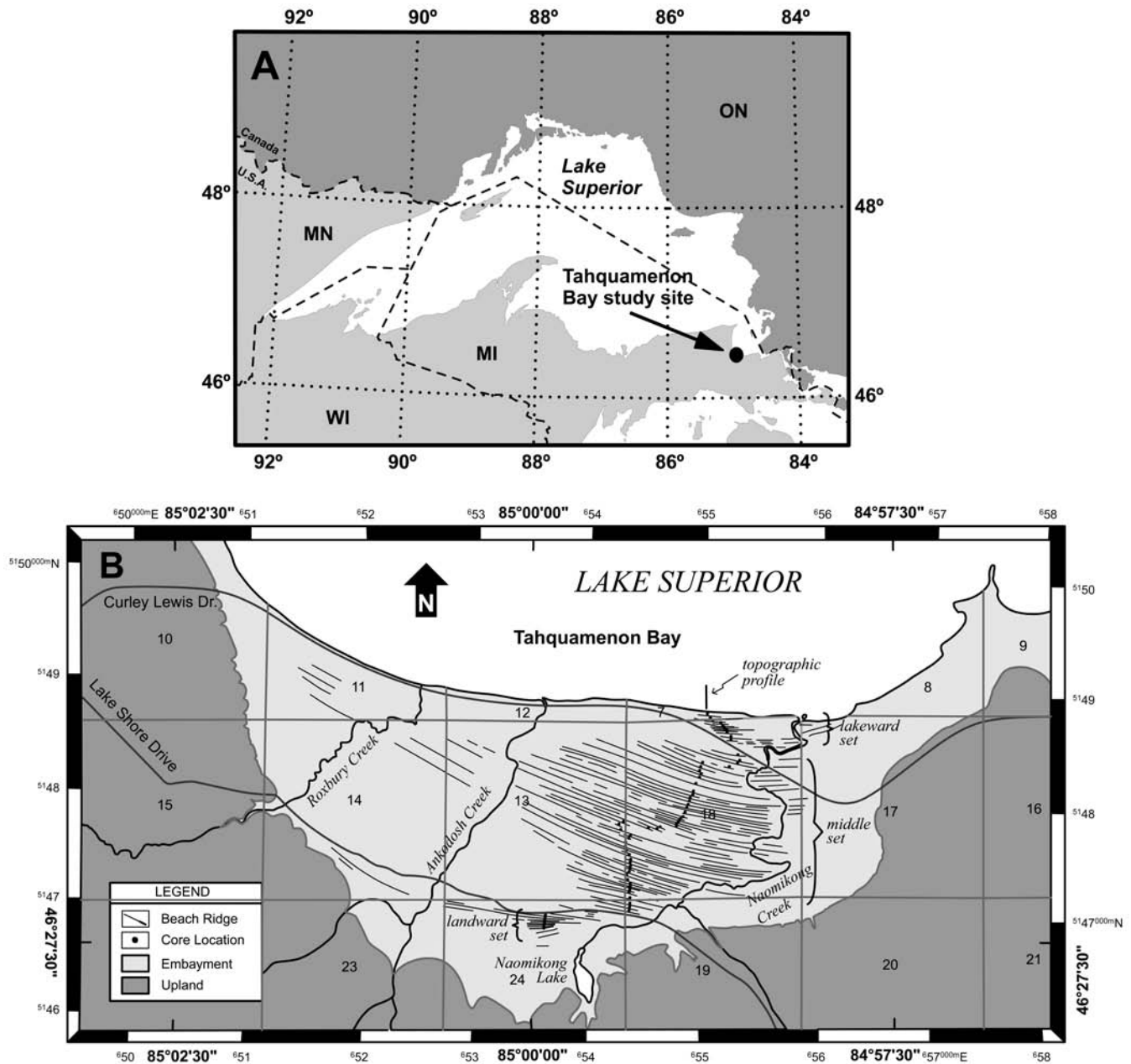
FIG. 1. Map showing the Tahquamenon Bay study area. (A) Map of Lake Superior showing the location of Tahquamenon Bay. (B) Map of the Tahquamenon Bay embayment. The lakeward side of 71 beach ridges were cored to determine the elevation of the lake when each beach ridge formed. Lines indicate beach-ridge crests and dots indicate core locations.
