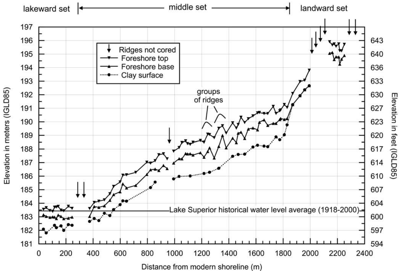
FIG. 4. Graph of the elevation of upper and lower limits of foreshore sediments versus distance landward from the modern shoreline. The middle line represents the boundary between foreshore and upper shoreface deposits and approximates the elevation of the lake during beach-ridge formation. The uppermost line represents the boundary between dune and foreshore deposits and is used in conjunction with the middle boundary to calculate foreshore thickness. The lowermost line corresponds to the contact between upper shoreface sediment and the predepositional surface composed of clay.
