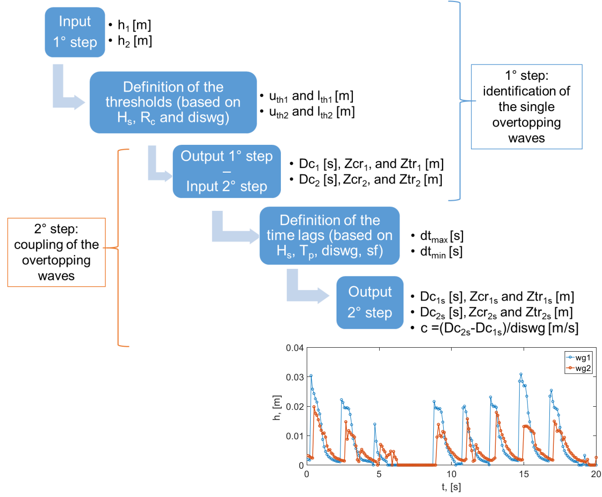
273 Figure 4 – Conceptual layout of the new procedure for the identification (1 st step) and the coupling (2 nd step) of the single wave overtopping 274 waves.
