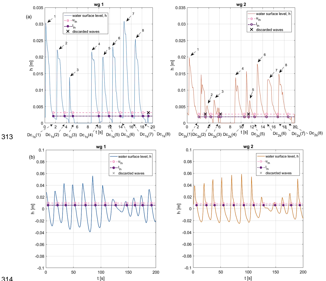
Figure 6 – h -signals measured at wg1 (left) and wg2 (right) at a dike at R_o/H_s=1 (panel a) and at R_o/H_s=-0.5 (panel b). The coupled events and the corresponding instants tdc are indicated and numbered (panel a). The discarded uncoupled events are marked with black crosses.
