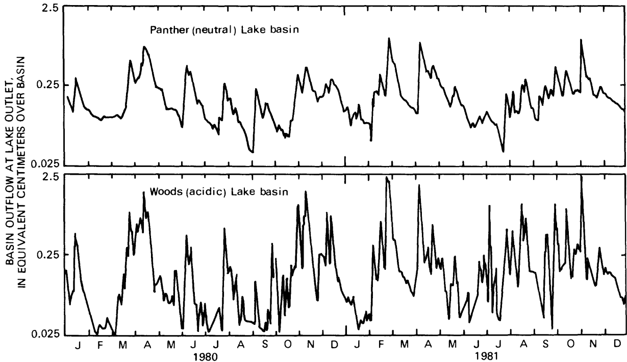
Figure 7.--Hydrographs of daily basin outflow, 1980-81.
