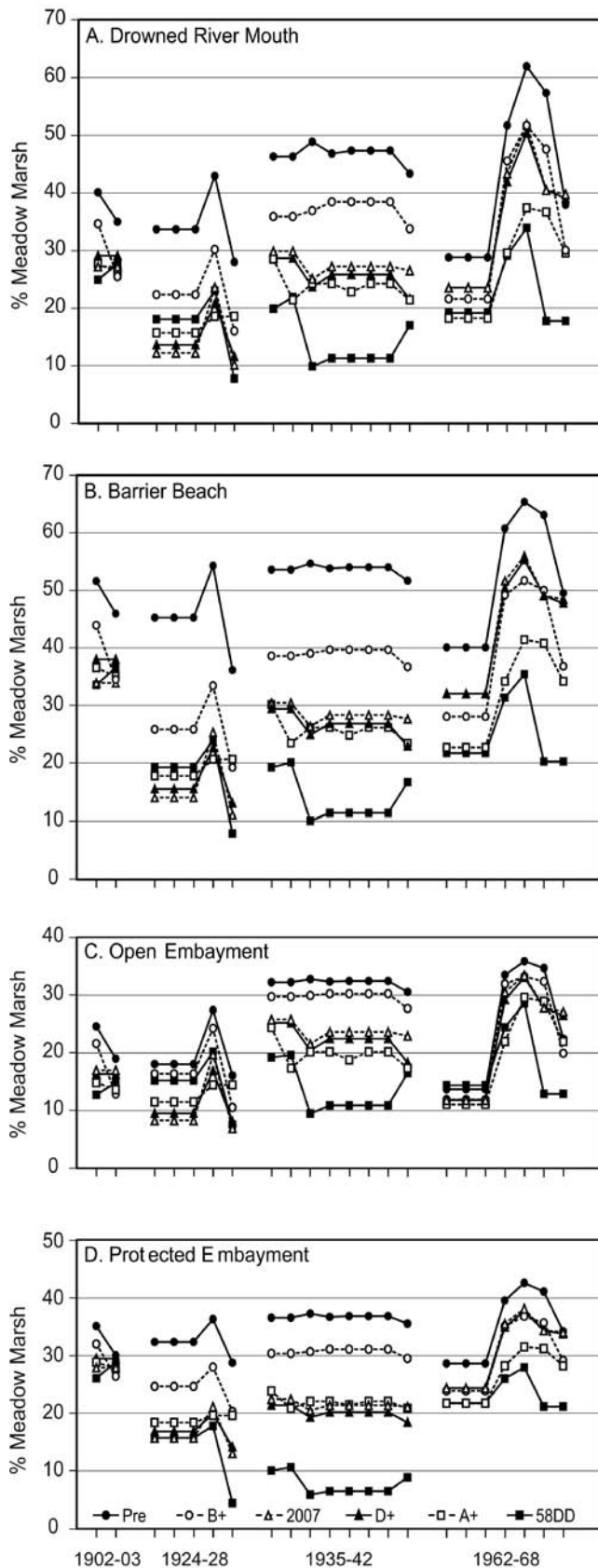
FIG. 2. Model-derived predictions of mean percent meadow marsh that would occur in Lake Ontario wetlands in years following low total basin supplies (1902–1903; 1924–1928; 1935–1942; 1962–1968) under simulated pre-regulation conditions and five lake-level-regulation plans. Wetland geomorphic types are a) drowned river mouth, b) barrier beach, c) open embayment, and d) protected embayment.
