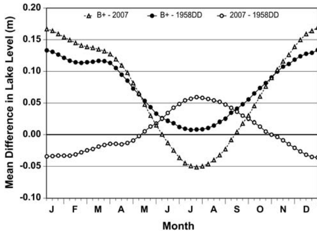
FIG. 3. Difference in mean water level of Lake Ontario by quarter months across 101 years (1900–2000) of total basin supplies when regulated by Plan B+ vs. Plan 2007 (B+ minus 2007 levels); Plan B+ vs. Plan 1958DD; and Plan 2007 vs. Plan 1958DD. In each evaluation, positive values reflect greater levels under the first plan, and negative values reflect greater levels under the second plan.
