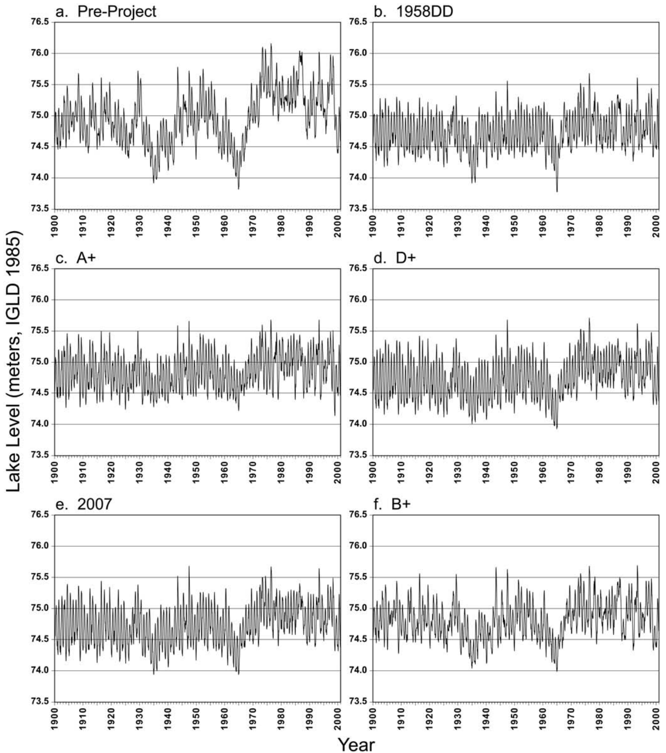
FIG. 1. Hydrographs provided by the International Lake Ontario-St. Lawrence River Study Board for Lake Ontario showing predicted lake levels for the period 1900-2000 based on total basin supplies with a) simulation of Pre-Project conditions with no regulation, b) regulation under Plan 1958DD, c) regulation under Plan A+, d) regulation under Plan D+, e) regulation under Plan 2007, and f) regulation under Plan B+.
