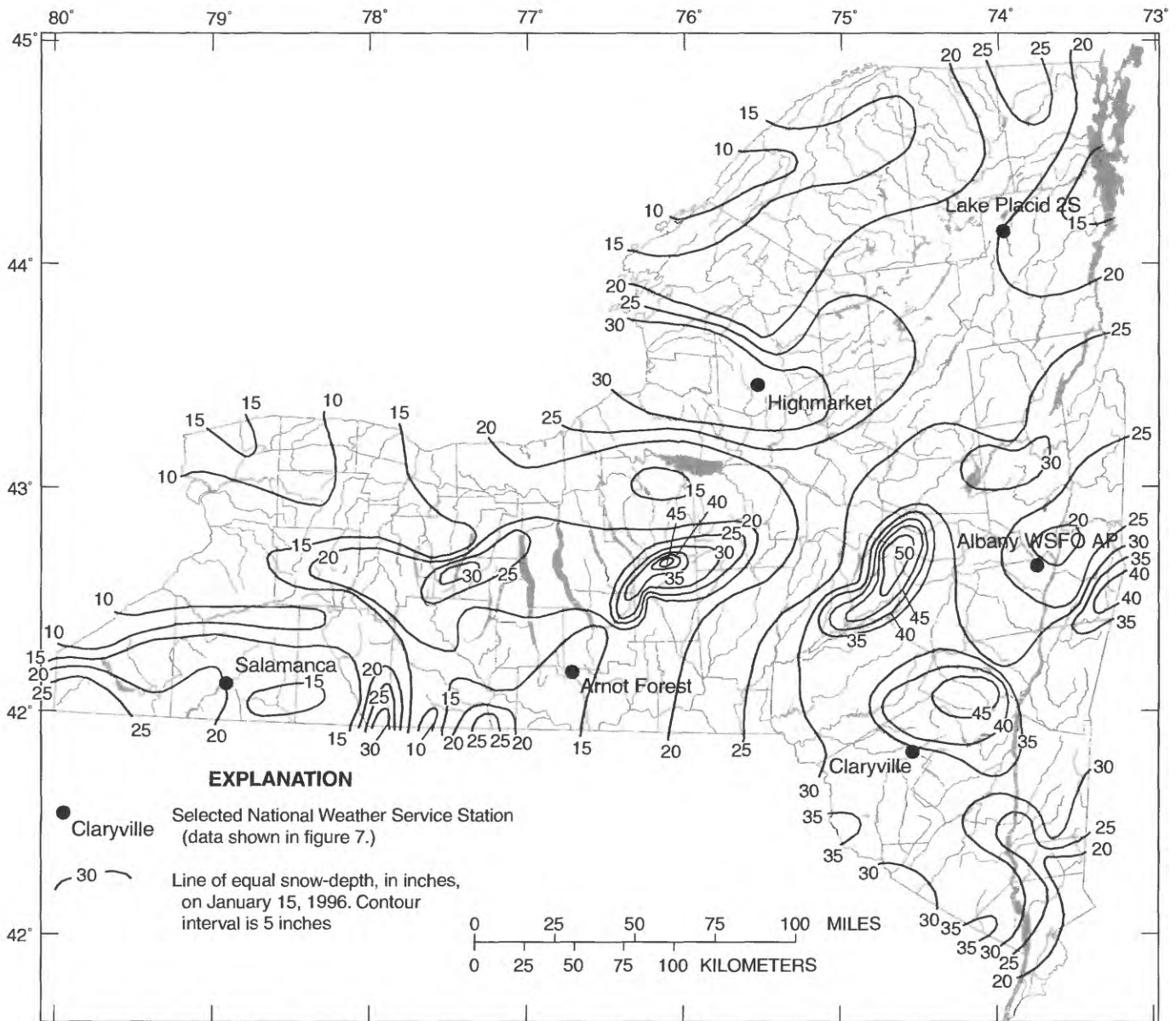
Figure 3. Lines of equal snow depth on January 15, 1996 in New York. (Data from National Oceanic and Atmospheric Administration, 1996).
