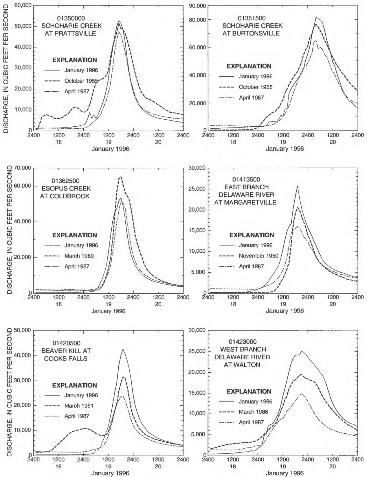
Figure 15. Discharge hydrographs of the January 1996 flood, the previous maximum flood, and the April 1987 flood at six continuous-record streamflow-gaging stations in the Catskill Mountain region of New York. (Locations are shown in fig. 10.)
