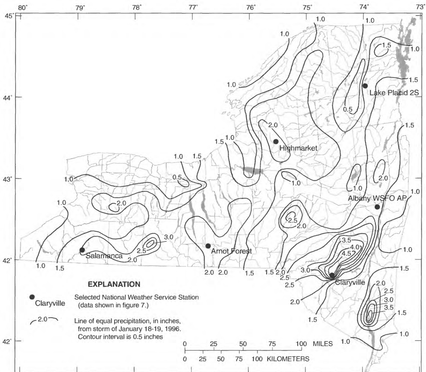
Figure 2. Lines of equal precipitation from the storm of January 18-19, 1996 in New York. (Data from National Oceanic and Atmospheric Administration, 1996).
