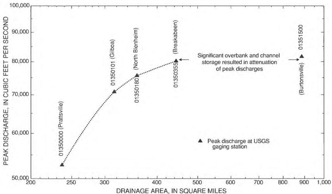
Figure 13. Peak discharge as a function of drainage area for sites on Schoharie Creek during the flood of January 19-20, 1996. (Locations are shown in fig. 10.)
