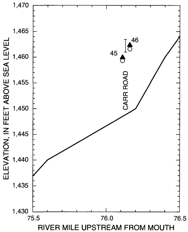
Figure 21 (continued) Water-surface profiles of Schoharie Creek during the flood of January 19-20, 1996.
