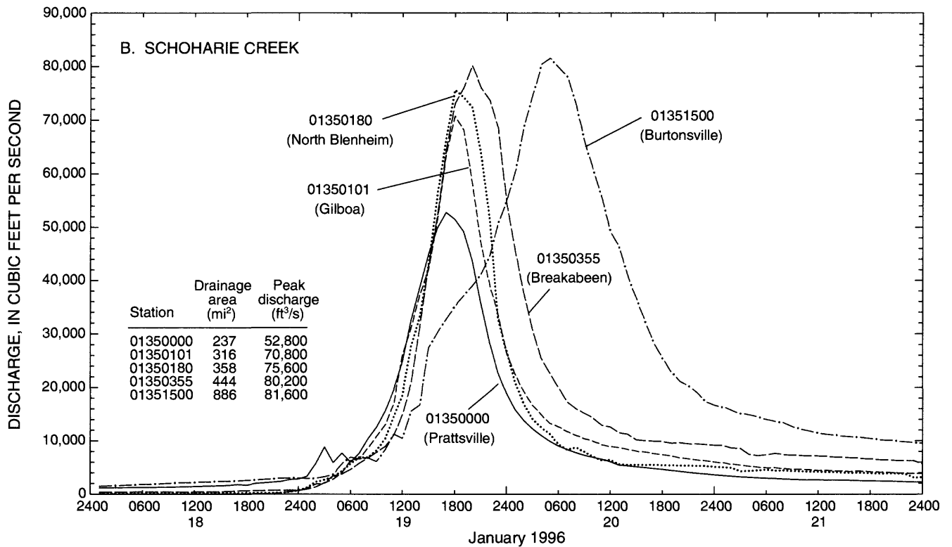
Figure 16. Discharge hydrographs for selected gaging stations in the Catskill Mountain region, N.Y., January 18-21, 1996. (Locations are shown in fig. 10; station names are given in table 5 at end of report.)
