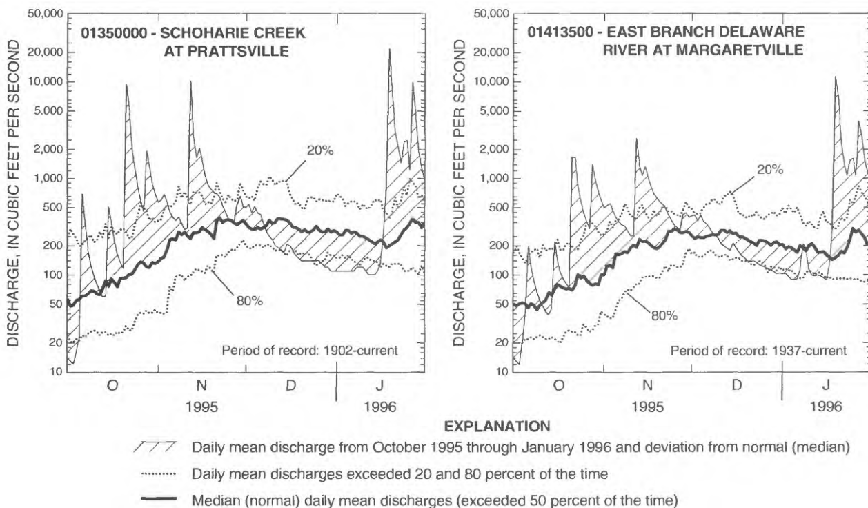
Figure 5. Daily mean discharges of two Catskill Mountain streams from October 1995 through January 1996., in relation to daily mean flows exceeded 20, 50, and 80 percent of the time. (Locations are shown in fig. 10.)
