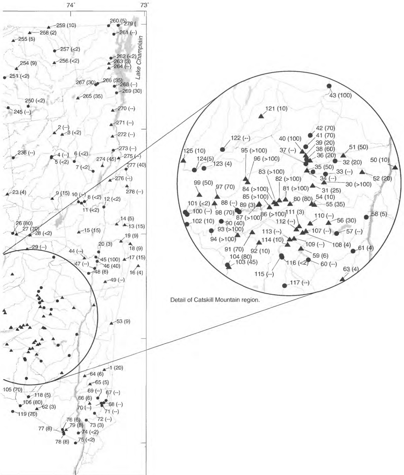
Figure 10. (Continued) Locations of streamflow gaging stations and peak discharge recurrence intervals for the floods of January 19-20, 1996 in New York. (Data given in table 5 at the end of the report).
