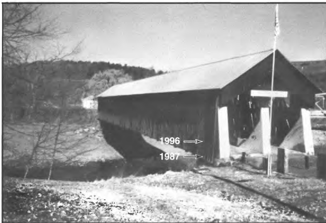
Figure 9D. Covered bridge over Schoharie Creek in North Blenheim, N.Y., with the height of the January 19, 1996 and April 1987 floods. (Photograph by Frank Dalton, U.S. Geological Survey, 1996.)
