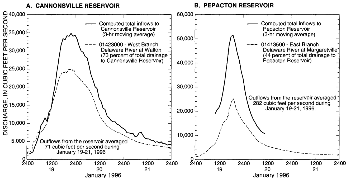
Figure 18. Inflows to Cannonsville and Pepacton Reservoirs during January 19-21, 1996. (Locations are shown in fig. 10.)
