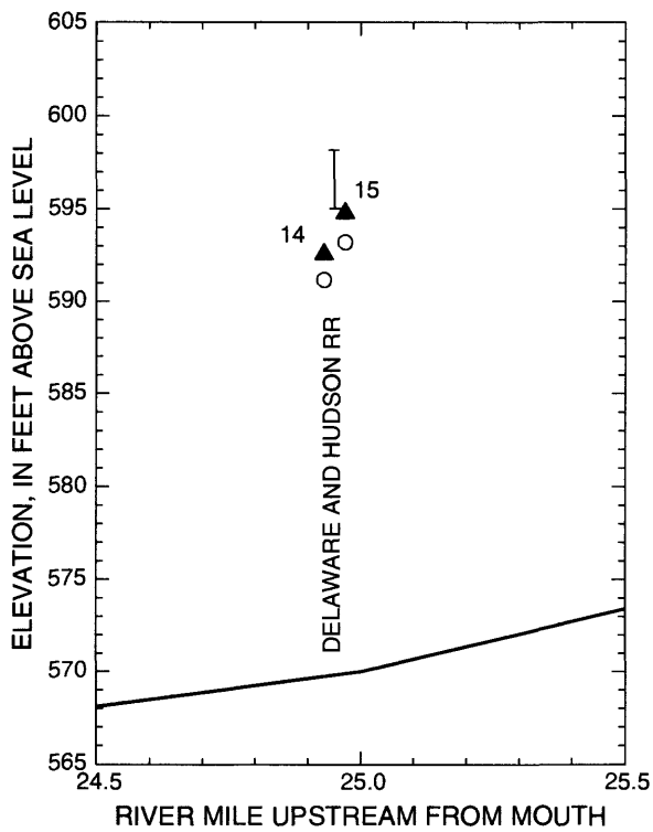
Figure 21. (continued) Water-surface profiles of Schoharie Creek during the flood of January 19-20, 1996.
