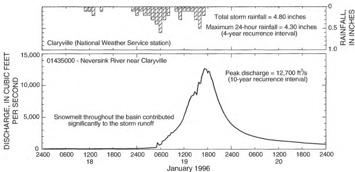
Figure 6. Rainfall and runoff at Claryville, N.Y., during the storm of January 18-20, 1996. (Locations are shown on fig. 2 and 10)
