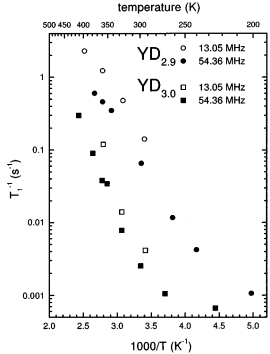
FIG. 7. Frequency dependences of T_1^{-1} of the YD_{3,0} and YD_{2,9} samples. The frequency dependence is approximately the same as for the NIST sample, as in Fig. 6.
