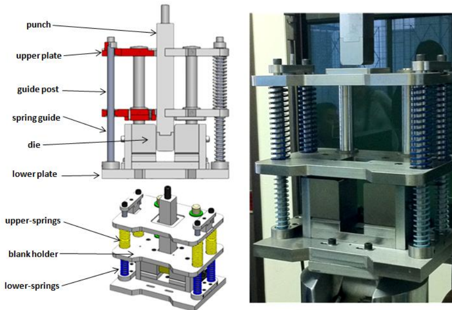
Figure 4: U-bending die experimental apparatus.
