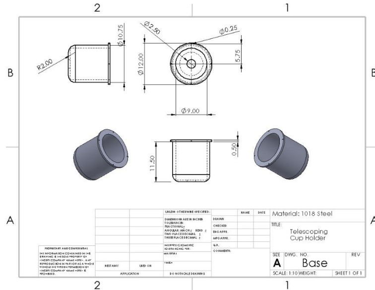
Figure 17: Base Drawing
