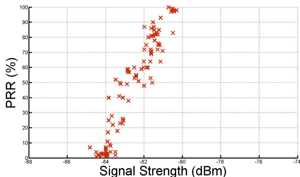
Figure 15. Relationship between signal strength and PRR, as measured experimentally.
