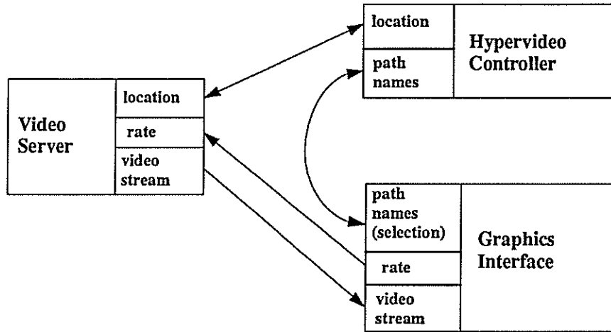
Figure 1: A hypervideo browser
