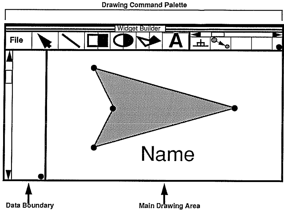
Figure 3: Graphical user interface editor
