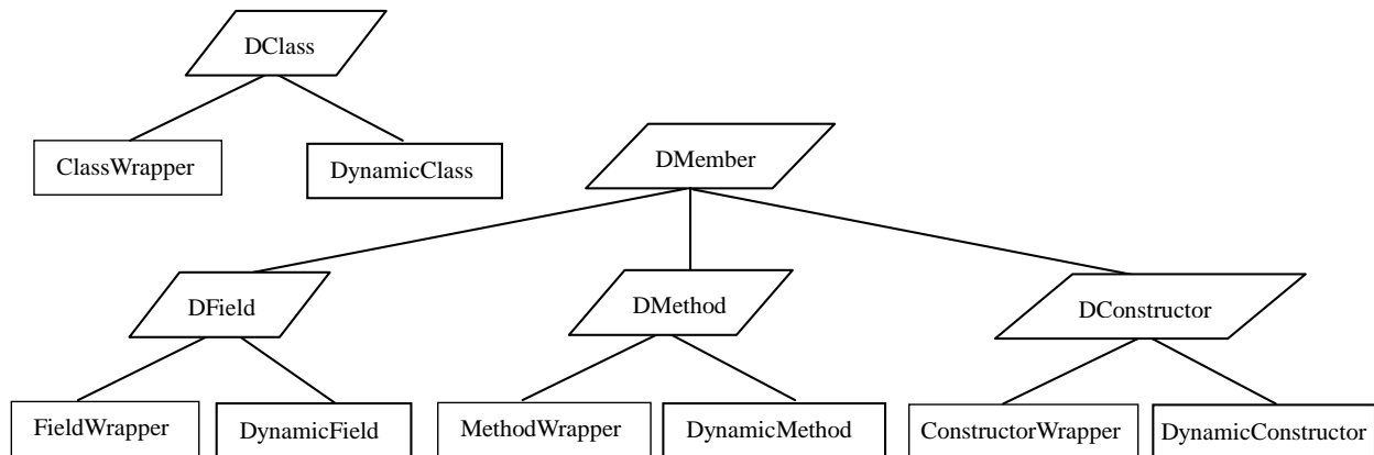
Figure 1: An integrated compiled and dynamic class reflection hierarchy.
