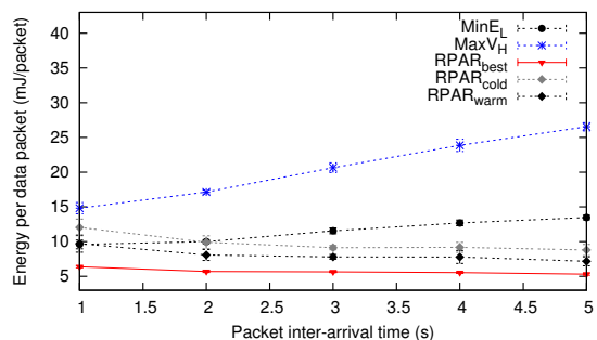
(d) Total energy consumption per data packet when data rate is varied
