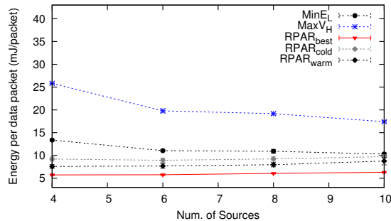
(b) Total energy consumption per data packet when number of sources is varied
