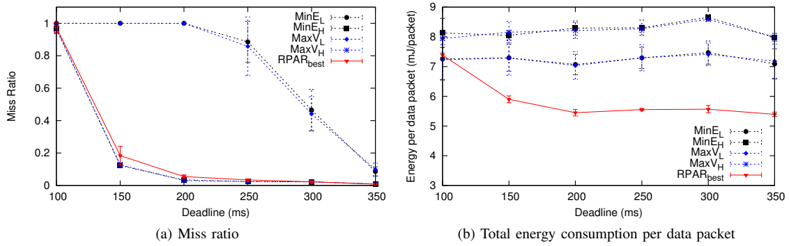
Fig. 2. Performance of considered protocols when deadline is varied. The neighborhood table is prefilled.
