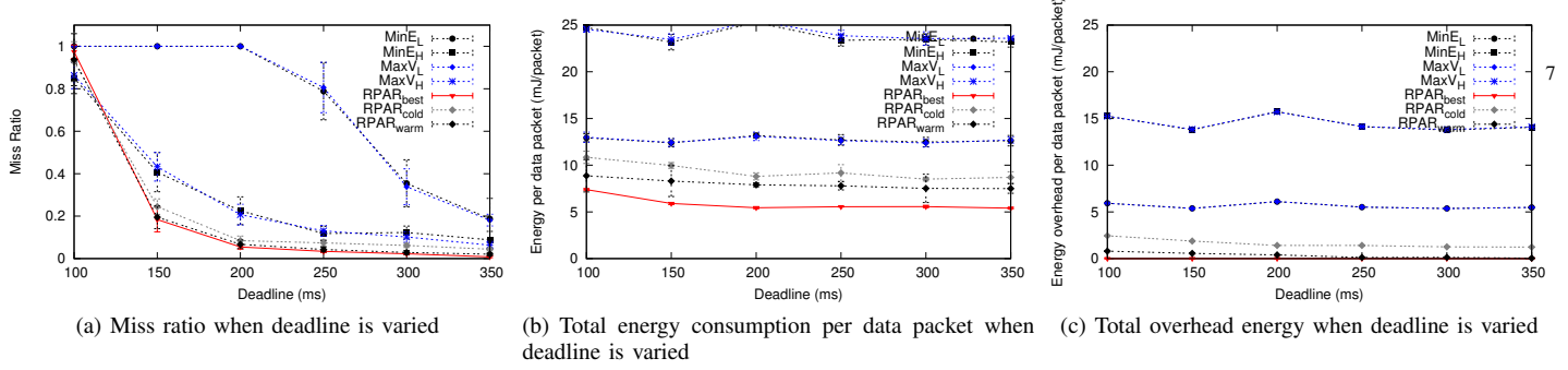
Fig. 3. Performance of considered protocols when deadline is varied (with neighborhood management).
