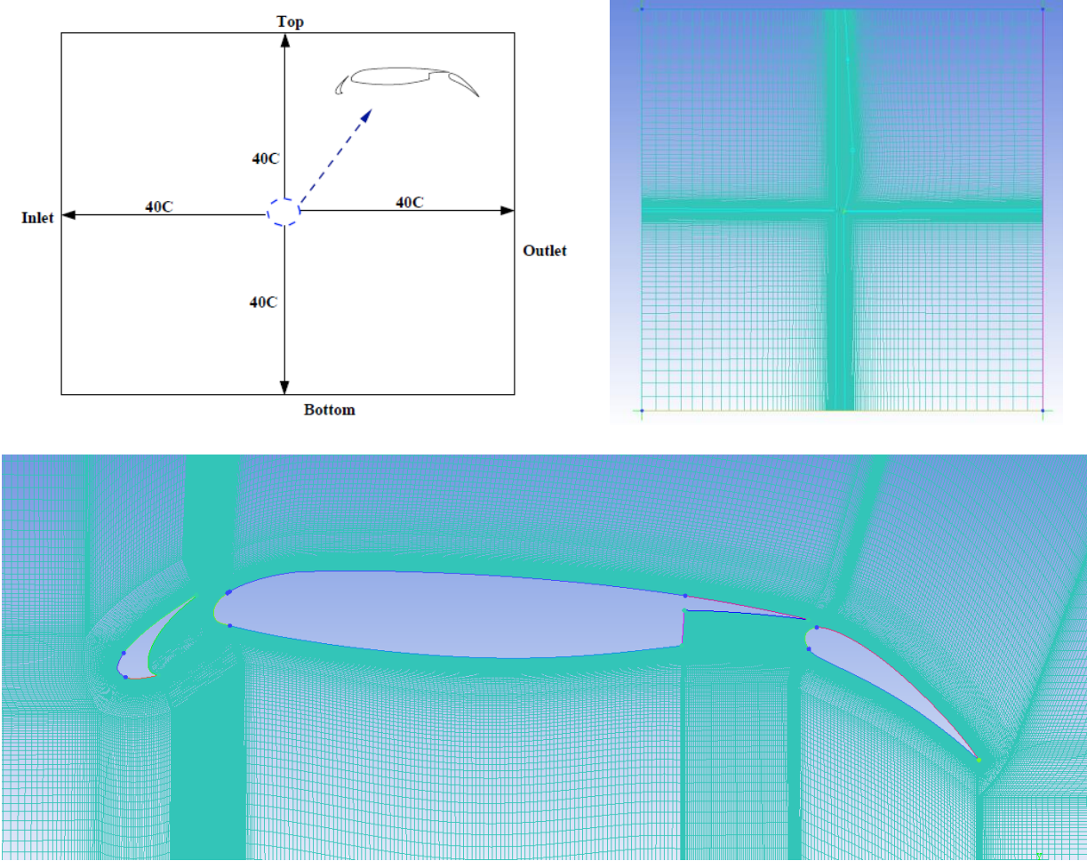
Fig 2.3 Computational domain and structured mesh layout in unbounded flow
