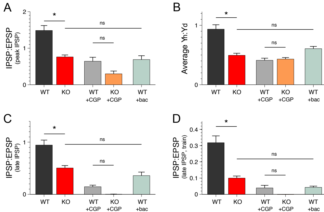
Figure 2.9. E/I imbalance in the FFI circuit of Fmr1 KO mice is GABA B receptor dependent.
