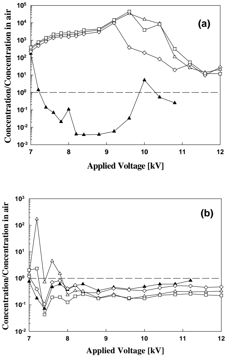
Figure 3.5: Ratio of concentration at ESP outlet when different gases are used to concentration at ESP outlet when air is used in the combustor, for (a.) positive applied voltages and (b.) negative applied voltages. Legend: \blacktriangle 50% O_2 -50% N_2 , \square 20% O_2 -80% CO_2 , \triangle 30% O_2 -70% CO_2 , \diamond 50% O_2 -50% CO_2 .
