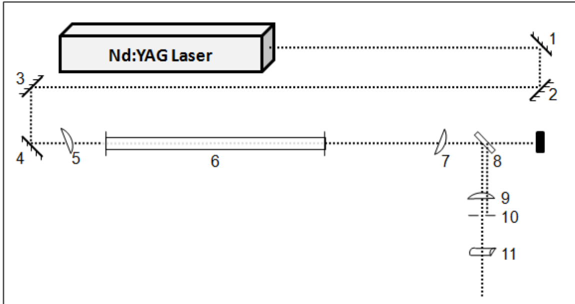
Figure 3.3: Schematic of the optic arrangement. 1-4, mirrors. 5, 7 and 9, lenses. 6, Raman shifter. 8, beam splitter. 10, aperture. 11, cylindrical lens.
