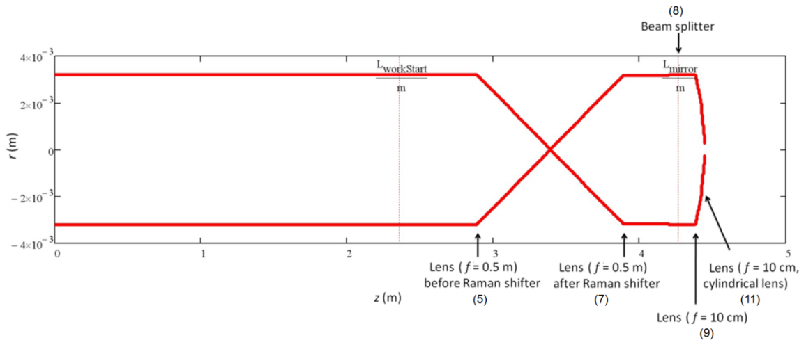
Figure 3.4: Beam envelop vs. beam path length. The optics are labeled as in Figure 3.3.
