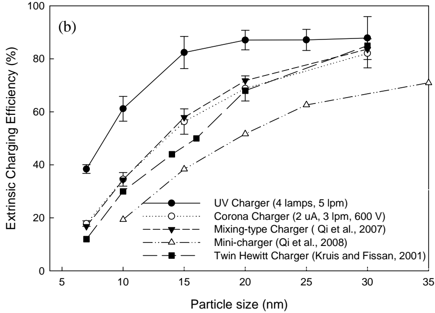
Figure 4.3 Comparison of intrinsic and extrinsic charging efficiency among different chargers for Ag particles in the size range from 7 to 30 nm
