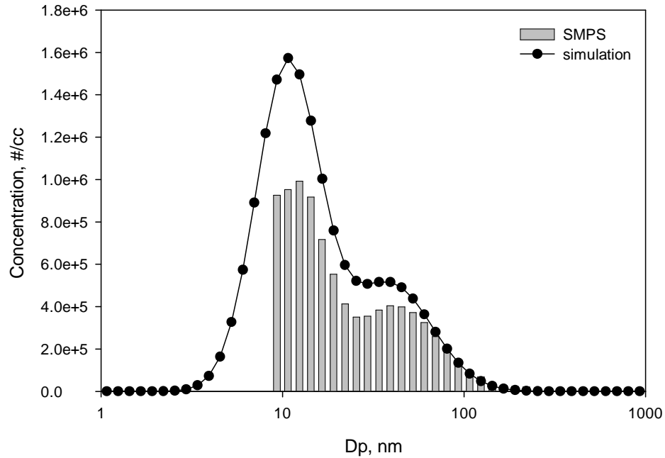
Figure 9 Comparison of bimodal particle size distributions measured by SMPS and retrieved by the proposed data-reduction scheme
