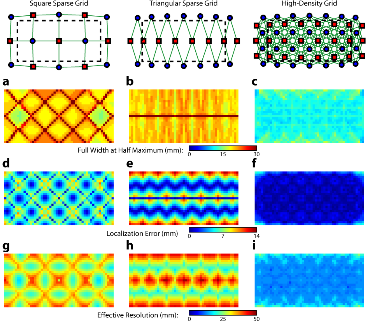
Figure 3.4: Image quality metrics for the point-spread functions of targets placed at every location in sparse and high-density grids. (a-c) Full width at half maximum of the imaging arrays. For the sparse arrays, there is overall poor resolution (high FWHM) with worse resolution along lines of symmetry in the grid geometry. Also, note that the triangular array has the worst resolution directly beneath the source line, where the system cannot constrain the activation vertically. The resolution for the high-density array is high (low FWHM) across the entire imaging domain with little variation. (d-f) Localization error of the imaging arrays. While the sparse arrays have low localization error directly under measurements and along points of symmetry, between measurements it is high. Localization error for the high-density array is uniformly low across the entire field-of-view. (g-i) Effective resolution of imaging arrays. The sparse arrays have poor effective resolution between the measurements, and only good effective resolution directly between adjacent sources and detectors. Effective resolution for the high-density array is good across the entire imaging domain, with little variation.
