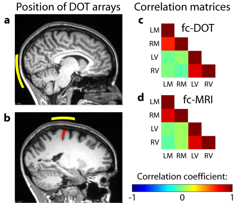
Figure 5.10: Comparing fcDOT with fcMRI. (a) Sagittal slice (5 mm left of mid-line) from subject's anatomical MRI with schematic of the visual cortex DOT pad superimposed (yellow), showing its position over the visual cortex. (b) Sagittal slice (18 mm left of midline) from an anatomical MRI with schematic of the motor cortex DOT pad superimposed (yellow), showing its position over the central sulcus (red). (c) Cross-correlation matrix for all four seeds from fcDOT imaging (LM: left motor cortex, RM: right motor cortex, LV: left visual cortex, RV: right visual cortex). Note the high inter-hemispheric correlations and low correlations between the motor and visual networks. (d) Cross-correlation matrix for all four seeds from fc-fMRI imaging. Note the similarity to the fcDOT correlation matrix.
