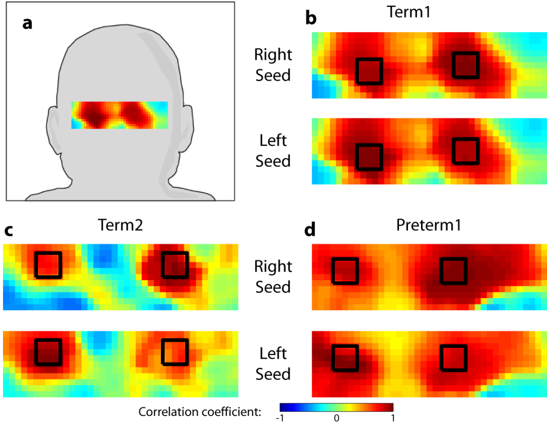
Figure 6.3: Neonatal fcDOT using correlation analysis in the visual cortex (HbO 2 ). (a) An fcDOT map placed over the occipital cortex of an infant head to show the field- and direction-of-view. (b-c) Correlation maps using seeds placed in the two visual hemispheres in healthy term infants. Note the strong ipsilateral and contralateral correlations. (All correlation images are scaled from r = -1 to 1.) (d) Correlation maps in the visual cortex of a healthy preterm infant, which also show strong bilateral correlation patterns.
