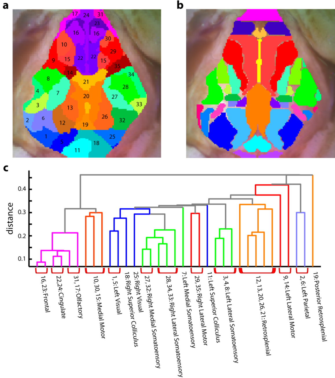
Figure A.11: Iterative parcellation with square tile seeding. (a) The results of iterative parcellation using 20 \times 20 pixel boxes as initial seeds. Although, the parcels are smaller, we can add them together to see the same networks as previously. (b) The Paxinos atlas applied to the mouse brain for comparison. (c) Clustering of the parcels from their parcel-to-parcel correlations. Branches are color-coded based on their functional assignments. The same general clustering patterns are noted. Perhaps since smaller parcels lead to some seed time traces having significant local vascular noise, some regions do not cluster as well, but most functional regions remains tightly grouped.
