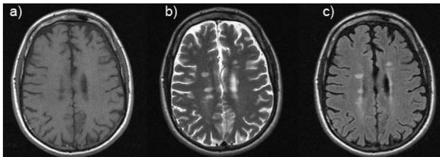
Figure 1.6 Example of clinical standard MRI used for monitoring MS (obtained in our laboratory). a) T1-weighted image, b) T2-weighted image, c) FLAIR.
