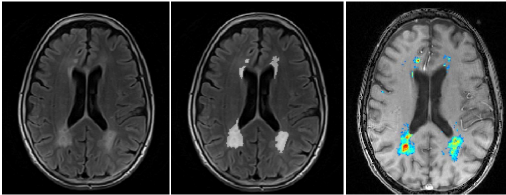
Figure 5.4 Illustration of GEPCI score maps obtained from subjects with RRMS and SPMS. They are made by overlapping colored TDS indices on T1 weighted images.
