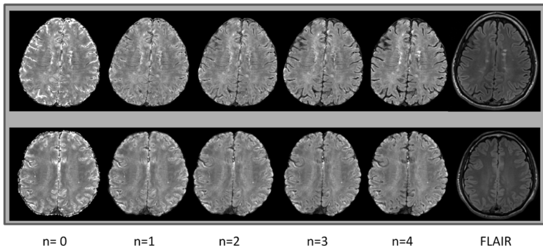
Figure 4.8 Example of the FST2* images (obtained using Eq. [4.9] with different parameter n ), and corresponding FLAIR T2 images. Top row – images from a subject with relapsing remitting MS, bottom row - images from a healthy subject.
