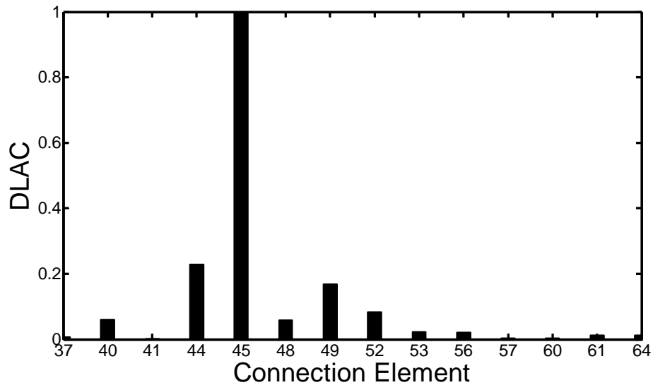
Figure 5.13 DLAC Values used for Localization of Damage Case 1
