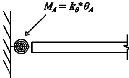
Figure 5.8 Common Modeling Approach for Semi-rigid Connections
