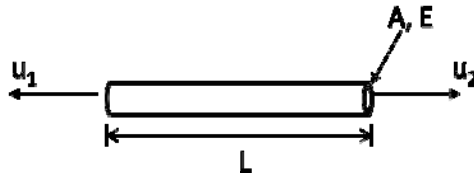
Figure 2.1 Two Dimensional Truss Element Degrees of Freedom
