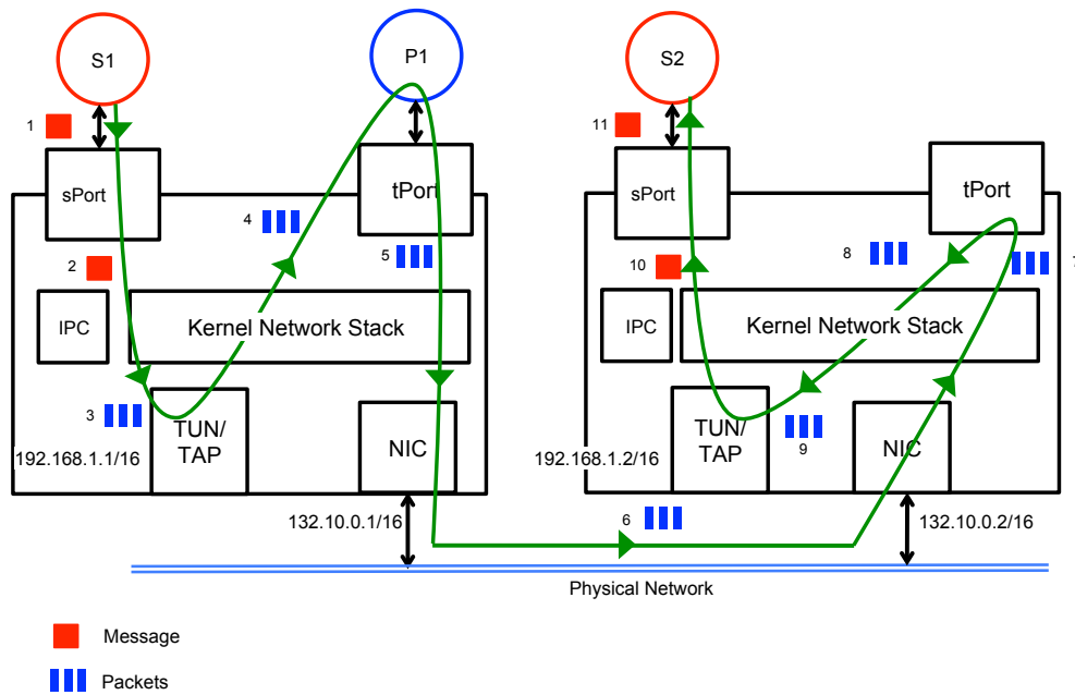
Figure 6.20: Case 4: Between two message-level services on different hosts thorough a packet level service
