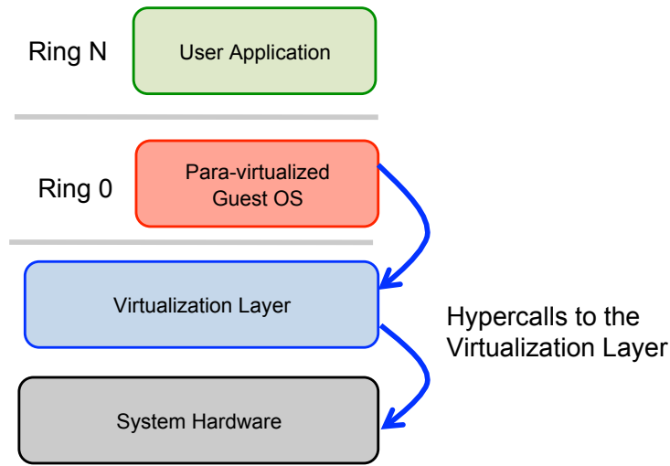
Figure 2.5: Para-Virtualization
