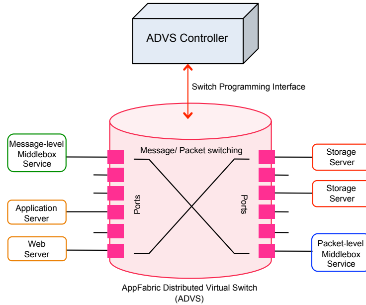
Figure 4.1: AppFabric Distributed Virtual Switch (reproduction of Fig. 3.4 )
