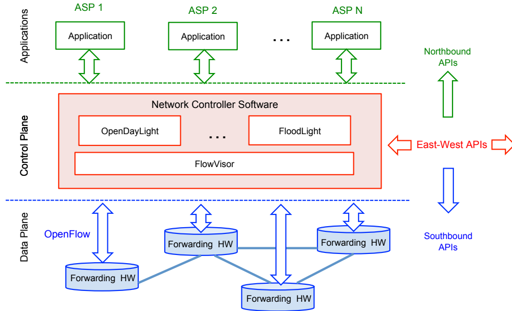
Figure 2.2: Software Defined Networking (SDN) Architecture
