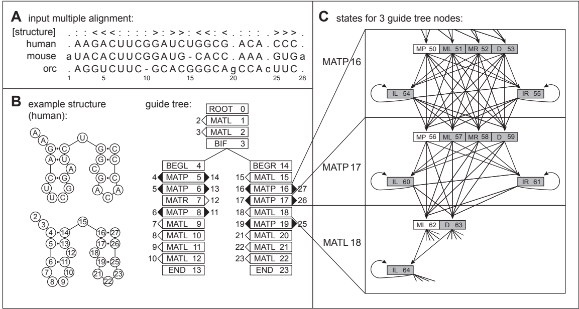
Figure 2.1: An example RNA family and corresponding CM. (A): A toy multiple alignment of three RNA sequences, with 28 total columns, 24 of which will be modeled as consensus positions. The [structure] line annotates the consensus secondary structure: < and > symbols mark base pairs, :’s mark consensus single stranded positions, and .’s mark “insert” columns that will not be considered part of the consensus model because more than half the sequences in these columns contain gaps. (B): The structure of one sequence from (A), the same structure with positions numbered according to alignment columns, and the guide tree of nodes corresponding to that structure, with alignment column indices assigned to nodes (for example, node 5, a MATP “match-pair” node, will model the consensus base pair between columns 4 and 14). (C): The state topology of three selected nodes of the CM, for two MATP nodes and one consensus “leftwise” single residue bulge node (MATL, “match-left”). The consensus pair and singlet states (two MPs and one ML) are white, and the insertion/deletion states are gray. State transitions are indicated by arrows.
