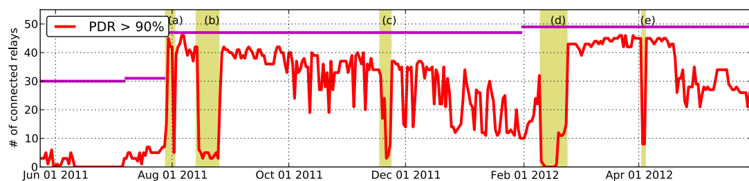
Figure 4.1 The network reliability from May 2011 to May 2012.
