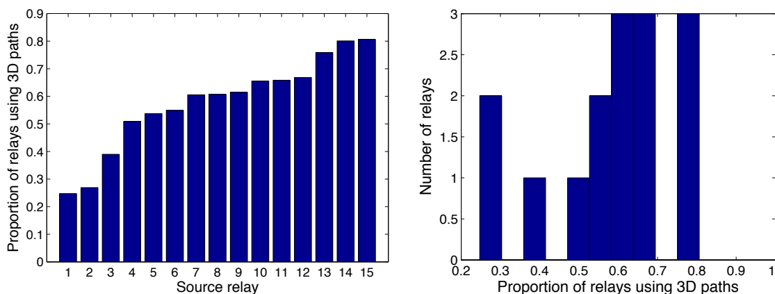
Figure 4.4 The proportion-of-time nodes on the 12 th floor used routing paths via the floor (ceiling). The left plot is ordered by proportion. The right plot is the histogram of the data, demonstrating that 12 relays out of 15 required 3D paths in more than 50% of their routes.
