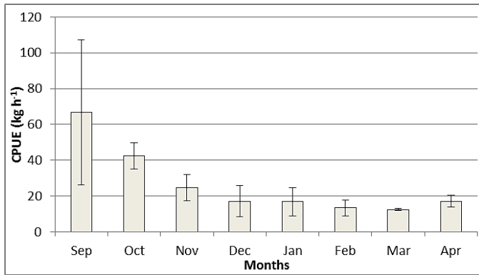
Figure 4. Time series of CPUE and standard deviations.
