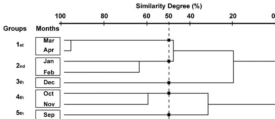
Figure 3. Catch composition similarity dendrogram according to monthly catch.
