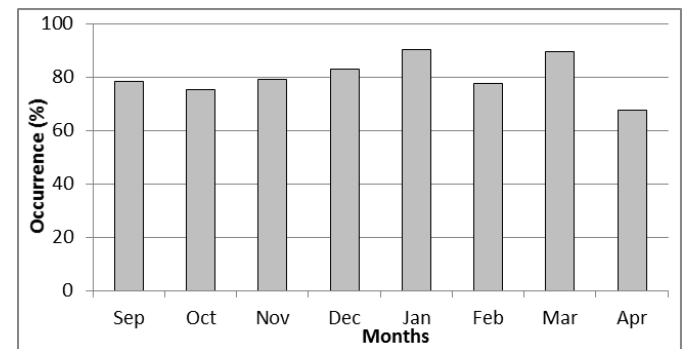
Figure 8. Monthly changes of percentage occurrence of fish in total catch.
