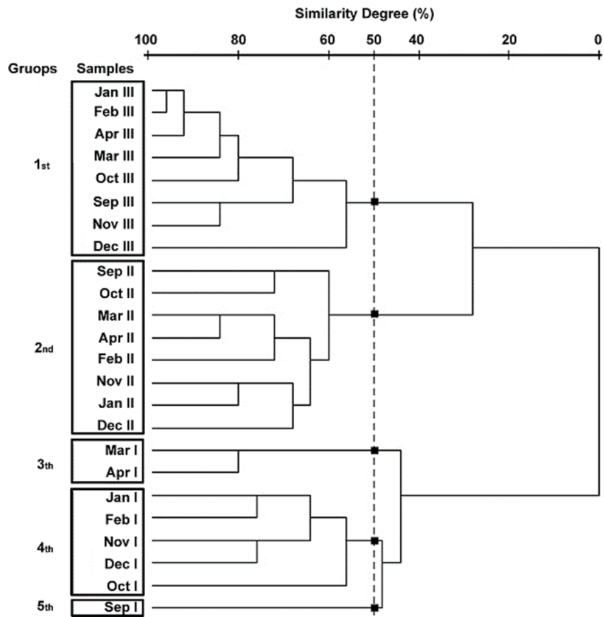
Figure 2. Catch composition similarity dendrogram according to depth ranges and months (I: 0-20 m; II: 20-50 m; III: 50-100 m depth range).
