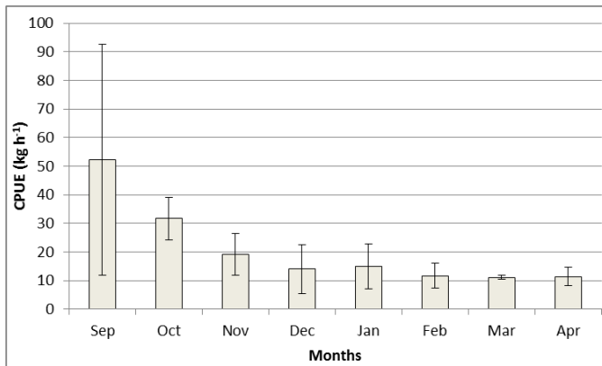
Figure 6. Mean monthly changes in the CPUE value of fish.
