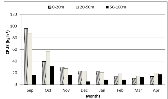
Figure 7. Monthly CPUE fishes in depth ranges.
