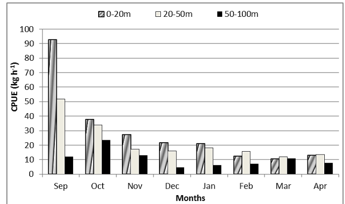
Figure 5. Monthly CPUE fishes in depth ranges.
