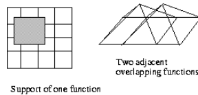
Figure 7: Reconstructing the value at a point on the surface. Resulting point is a linear sum of the four functions overlapping at any given point.
