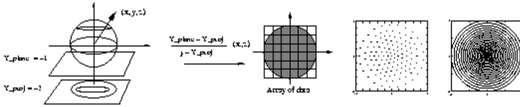
Figure 3: Projecting from the hemisphere of directions to the plane. On the right we show the projection of two different data sets; an evenly distributed set of data points generated from an icosahedron, and concentric rings taken at evenly spaced longitudinal intervals \theta = \pi/2 to \theta = 0 .
