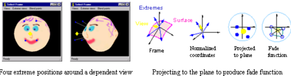
Figure 2: A view direction and its four extreme points. The fade function is constructed by projecting the points onto the plane and building a smooth “hat” function over the resulting polygon by placing the fade curve with its 1 end at the center of the projected view and its 0 end on the boundary of the polygon.
