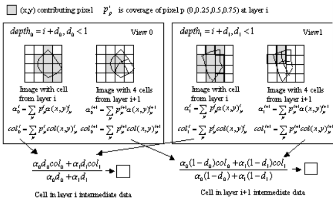
Figure 4: How data is blended from two overlapping views.
