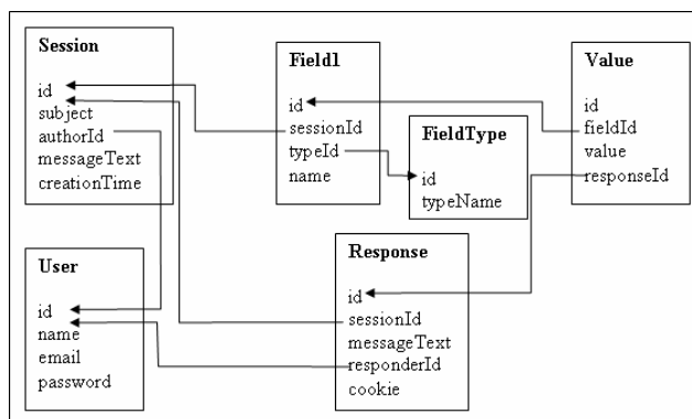
Figure 4. SmartMail database schema
