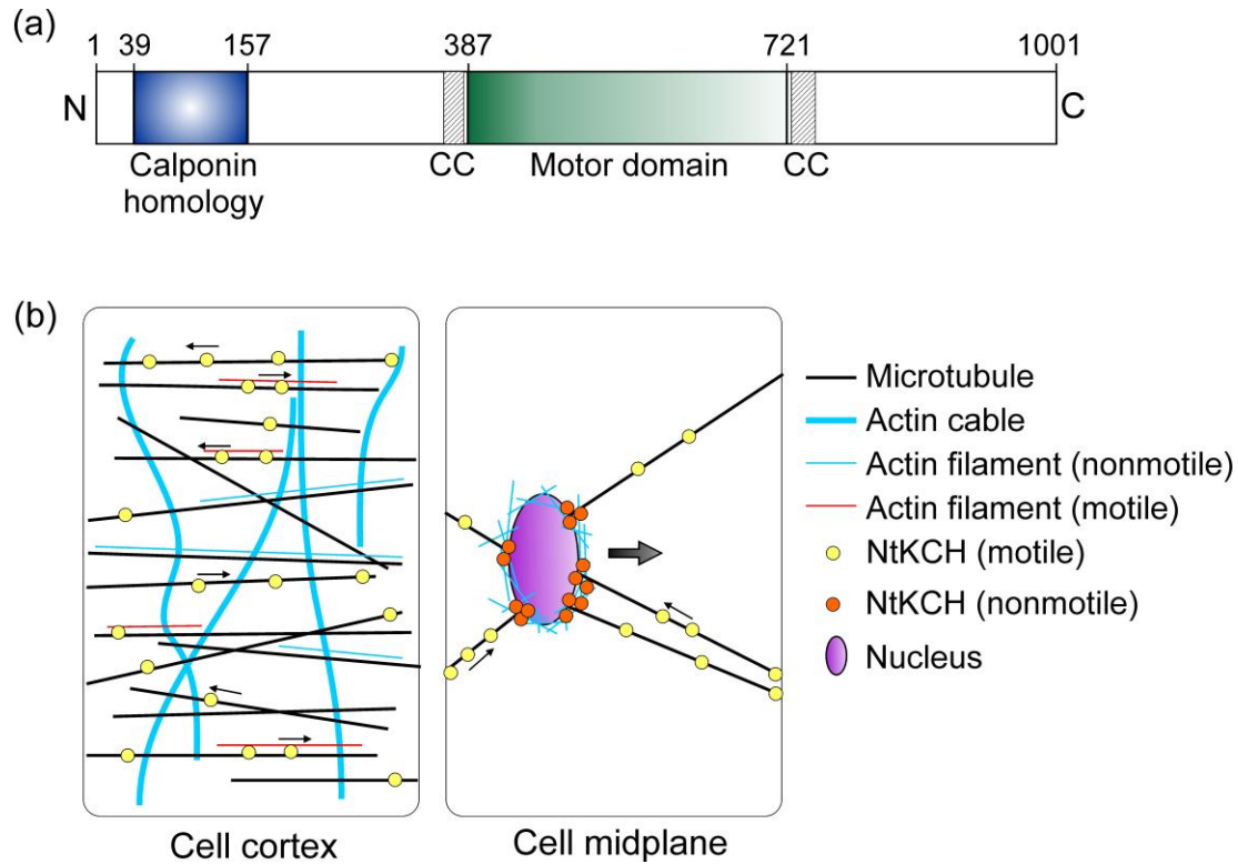
Fig. 1 NtKCH structure and cellular localization. (a) Domain structure of NtKCH. The N-terminal calponin homology domain mediates actin binding while the motor domain contains the MT and ATP binding sites. The motor domain is predicted to be flanked by coiled-coil (CC) domains, which might lead to dimerization. (b) Subcellular localization and proposed functions of NtKCH. During interphase, the cortical NtKCH population is motile (arrows) and might carry cargo such as actin fragments along cortical MT tracks. The perinuclear population of NtKCH is stably bound to actin and is nonmotile. The nonmotile NtKCH population is thought to tether the nuclear actin basket to MTs that extend from the nucleus to the cell cortex. Motile NtKCH molecules exist along these MTs and move inwards towards the nucleus. Cortical NtKCH molecules (or other kinesins) might exert pulling forces on these MTs, leading to movement of the nucleus towards the cell center (large arrow).
