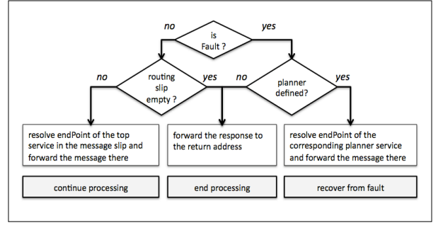
Figure 4: Routing algorithm
