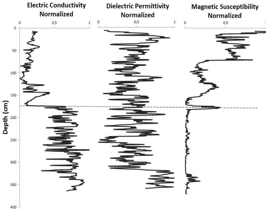
Figure 2. Normalized profiles of electric conductivity (left), dielectric permittivity (center), and magnetic susceptibility (right) as functions of depth.
