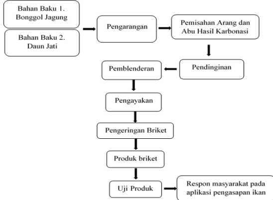
Gambar 1. Prosedur penelitian
