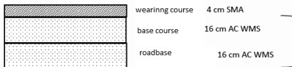
Fig. 4. Durable asphalt pavement cross-section Poznański model [6].
