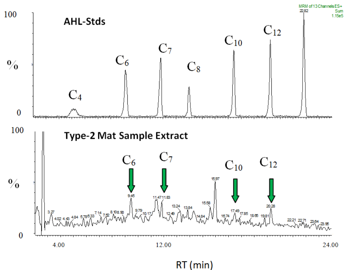
Figure 7. Spectra showing AHLs extracted from Type 2 mats, and AHL standards. Samples are separated using LC/MS. Peaks are shown as a relative percent (y-axis), while x-axis shows retention time (RT), expressed in minutes.
