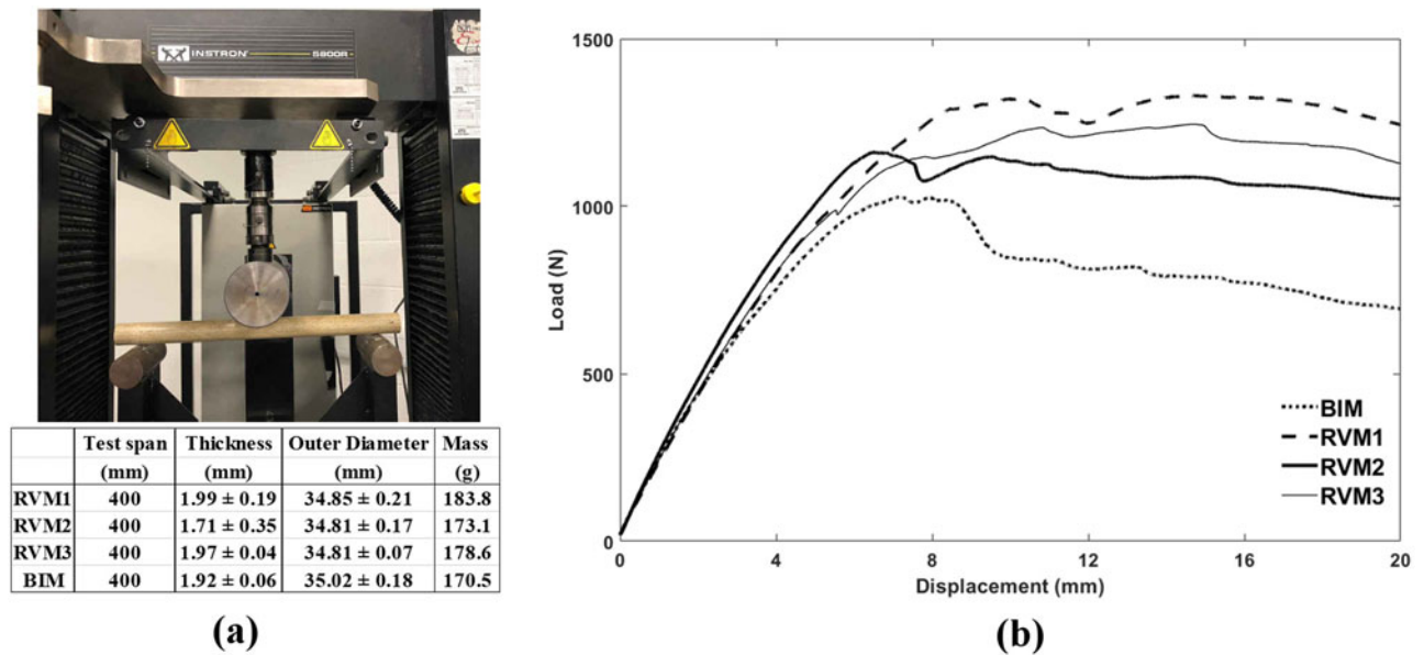
Figure 3. (a) Three-point flexure testing setup with specifications of test specimens; (b) Load-displacement response of the BIM and RVM beams.
