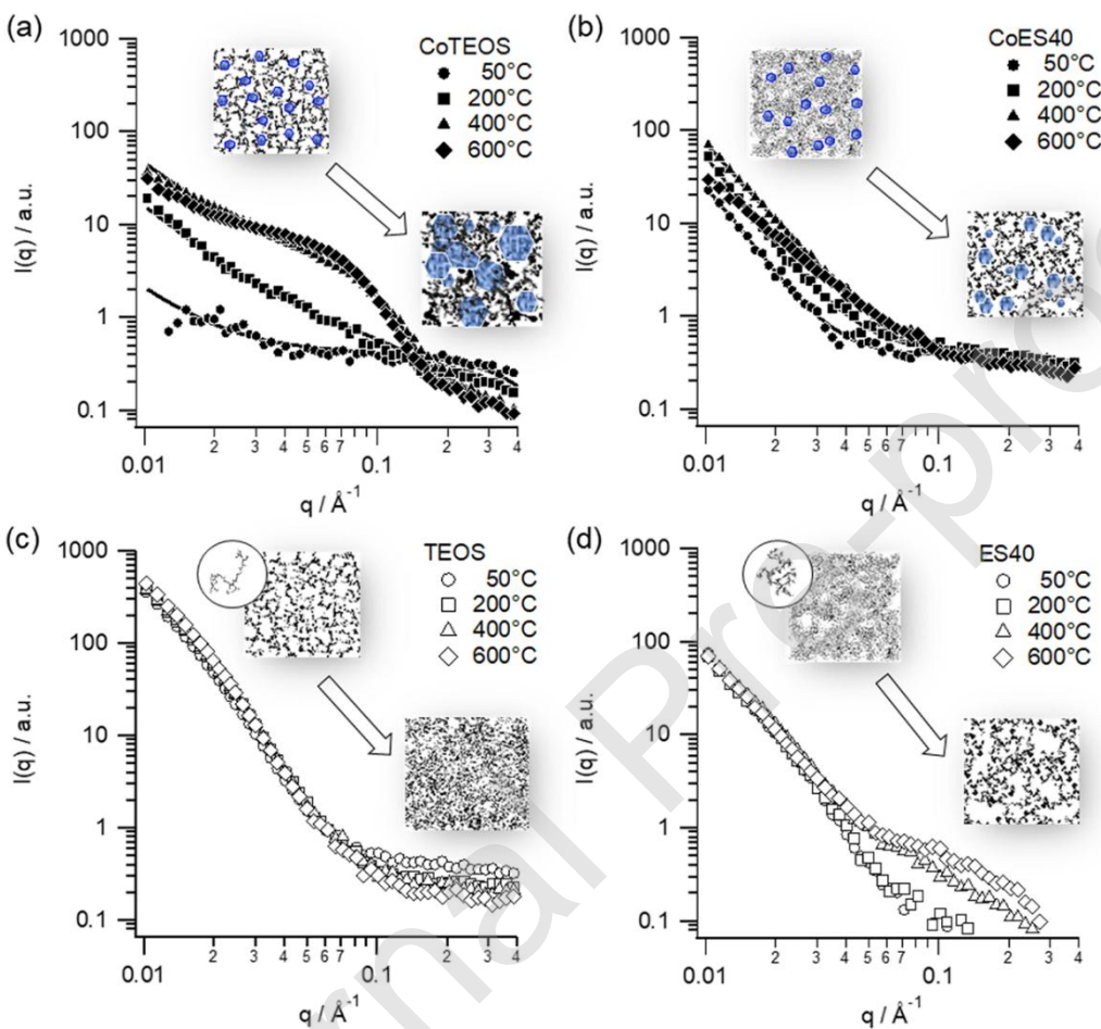
Fig. 4. Synchrotron in-situ SAXS patterns for (a) CoTEOS and (b) CoES40 nanocomposites with their fitting lines fit with a two-sphere plus mass fractal model ( R_{\text{sphere1}} = 5\text{\AA} plus R_{\text{sphere2}} = 22\text{--}28\text{\AA} ) and mass fractal model, respectively. Lines under data points are fits, uncertainties are within the size of the data points. For comparison, SAXS patterns for (c) TEOS- and (d) ES40-derived gels are provided.
