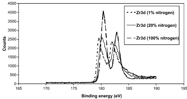
Fig. 5. Chemical shift of the Zr3d XPS peak with nitrogen.
