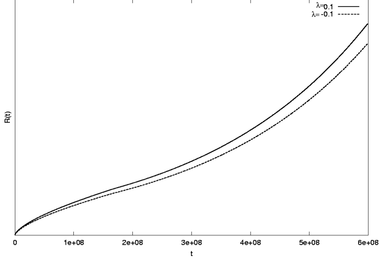
Figure 3: Expansion factor computed from Eqs. 49 and 43 illustrating the behaviour of an hypothetic universe filled with matter ( \omega = 0 ) and an exponentially harmonic map. ( \dot{\phi}_0 = 1 , \ddot{\phi}_0 = -5 , \omega = 0 ).
