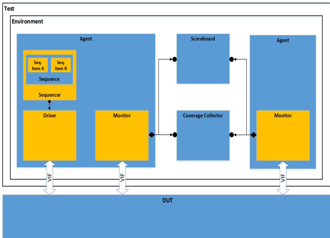
Figure 1. An example of a generic UVM test bench. The test bench resides within the test block and it communicates to the DUT via one or several virtual interfaces (VIF), here depicted as bidirectional arrows. The environment inside the test contains two agents , a scoreboard and a coverage collector . The leftmost agent contains a driver , a monitor and a sequencer . The sequencer further contains a sequence that is built on sequence items (Seq. Item A & Seq. Item B). The rightmost agent only contains a monitor and is called a passive agent as it does not drive any data to the DUT. The leftmost agent, by contrast, is an active agent.
