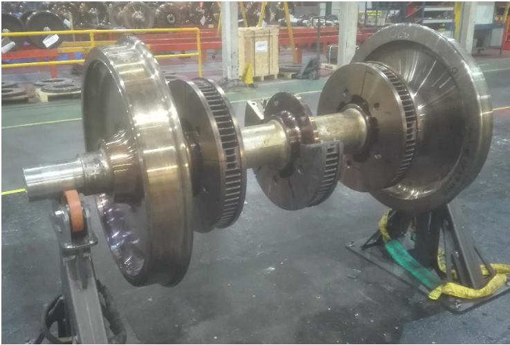
Figure 2 Wheelset equipped with segmented brake discs (only partially mounted segments).
