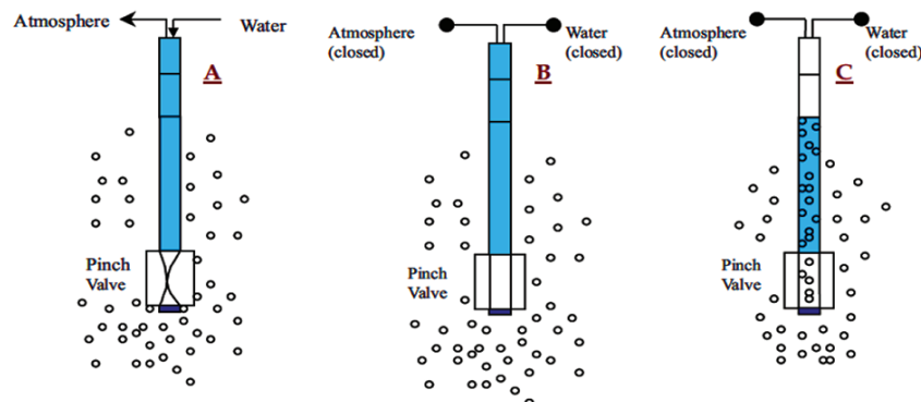
Figure 2—A schematic of steps to measure superficial gas velocity by J_g probe (Power, Franzidis, and Manlapig, 2000)
