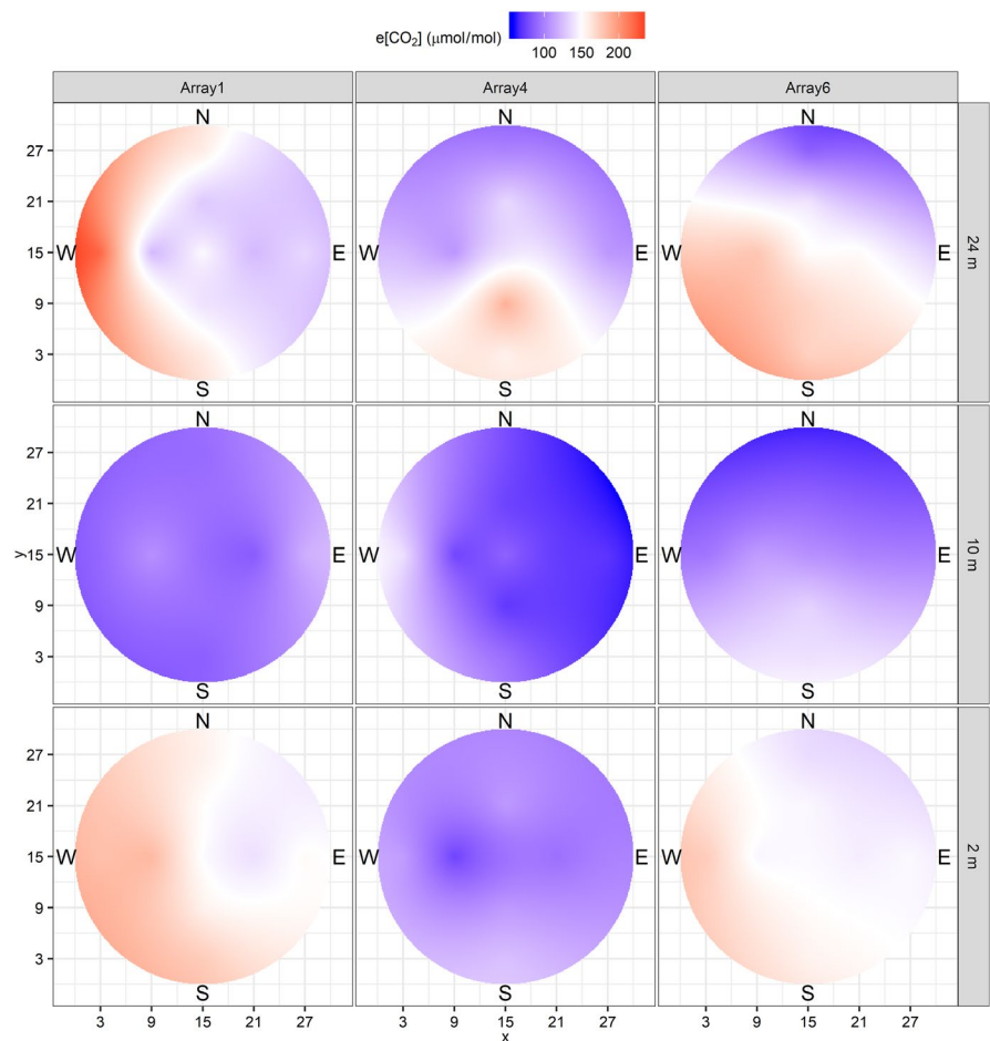
FIGURE 9 Interpolated mean distribution of e[CO 2 ] (μmol/mol) in the fumigated arrays for the 2017 season measured at three heights (m) from the ground (2, 10 and 24 m). X and Y axes units are meters (m) from the internal array edge. Kriging was performed after fitting a variogram using a linear model with partial sill = 1 and range = 0. The measurements informing this interpolated field are at 12, 6 and 0 m from array centre in the four cardinal compass directions
